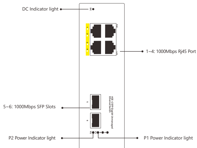
Front panel diagram
